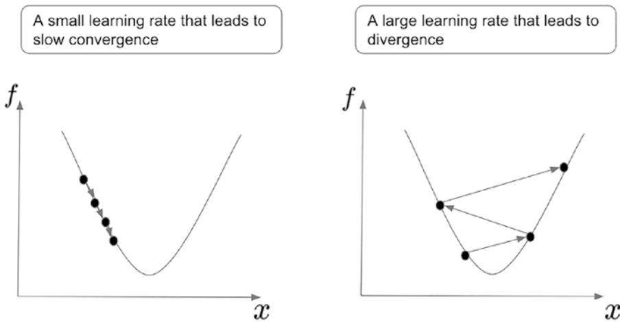
Figure 1-4. Slow convergence due to a small learning rate on the left and divergence due to a large learning rate on the right
