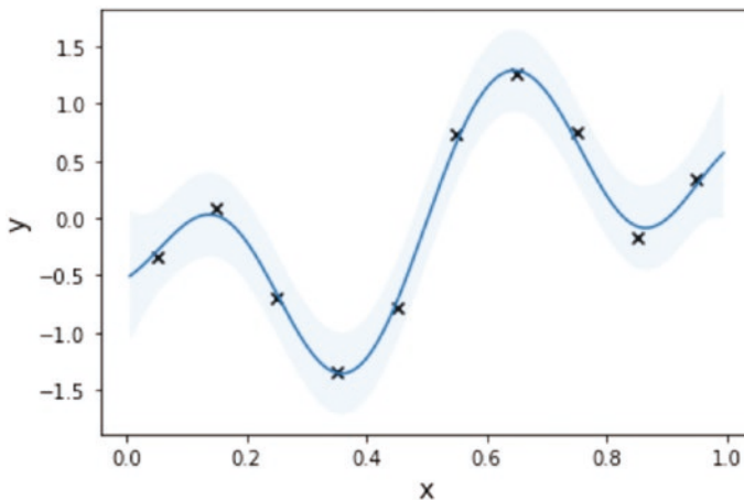
Figure 4-6. Visualizing the GP fit after optimizing model hyperparameters, that is, the length scale and noise variance
