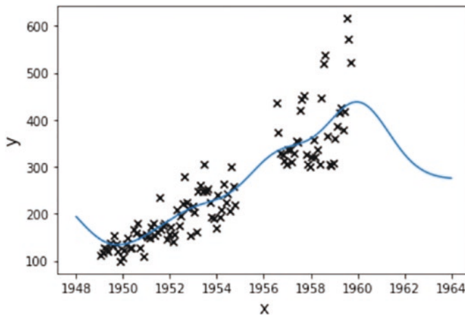
Figure 4-14. Visualizing the GP regression fit using the RBF kernel and polynomial kernel
