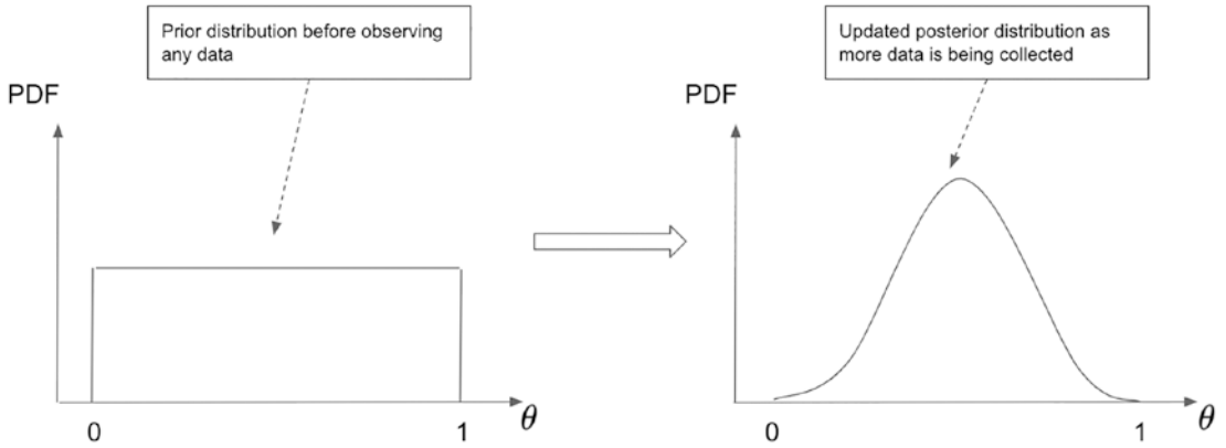
Figure 1-8. Updating the prior uniform distribution toward a posterior normal distribution as more data is collected. The role of the prior distribution decreases as more data is collected to support the approximation to the true underlying distribution
