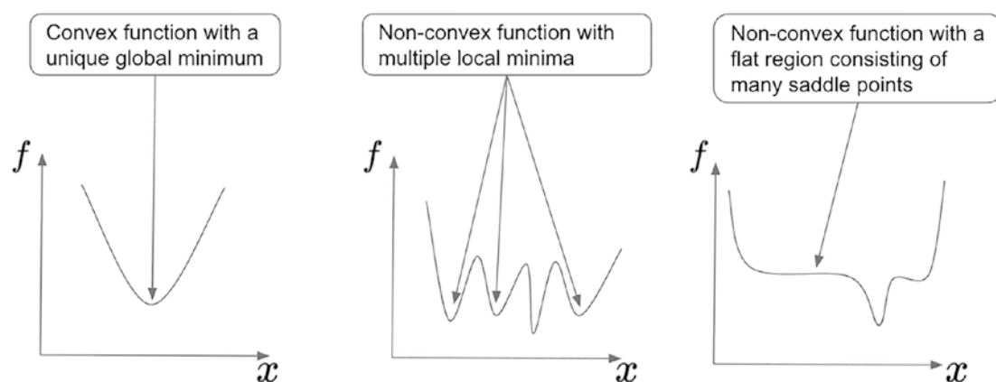
Figure 1-3. Three possible functional forms. On the left is a convex function whose optimization is easy. In the middle is a nonconvex function with multiple local minima, and on the right is also a nonconvex function with a wide flat region full of saddle points. Optimization for the latter two cases takes a lot more work than for the first case
