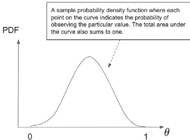
Figure 1-7. Illustrating a sample (continuous) posterior distribution for the parameter of interest. The specific shape of the curve will change as new data are being collected
