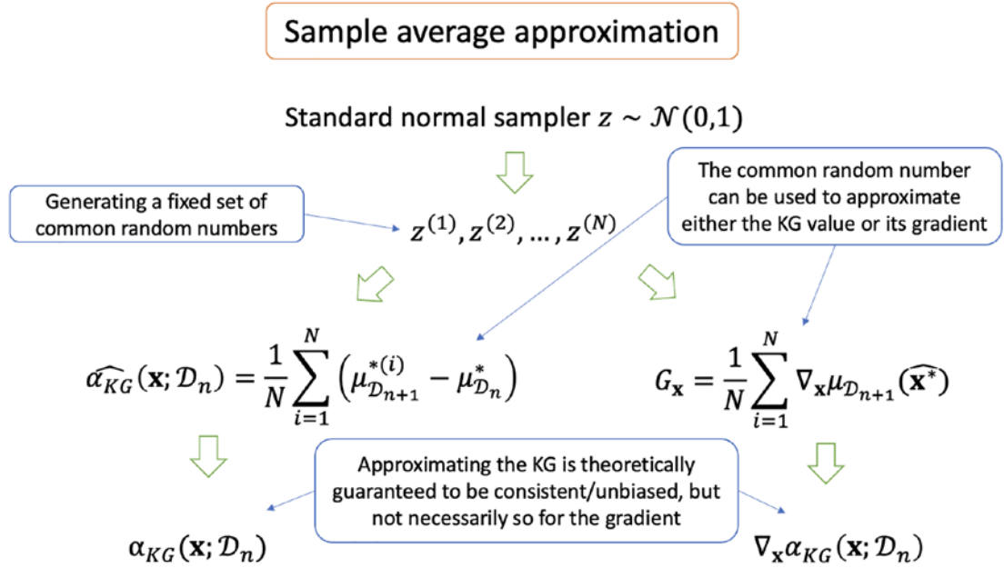
Figure 6-8. The sample average approximation technique used in the Monte Carlo estimation for both the KG value and its gradient estimator using quasi-Newton methods for faster convergence speed and more robust optimization
