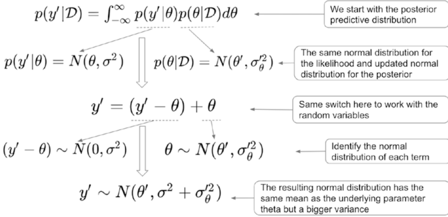
Figure 1-13. Derivation process of the posterior predictive distribution for a new data point after collecting some observations, assuming a normal distribution for both the likelihood and the prior
