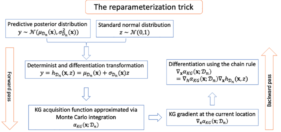
Figure 6-6. Illustrating the reparameterization trick for the gradient calculation of the KG acquisition function
