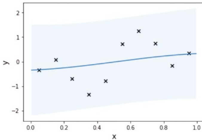
Figure 4-3. Visualizing the fitted GP regression model
