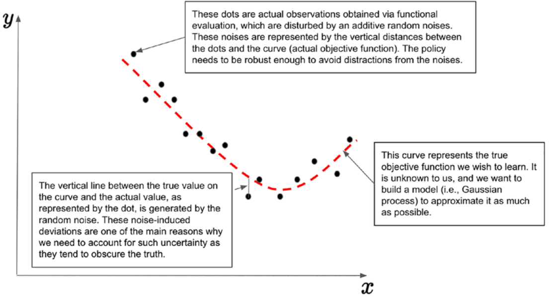
Figure 1-5. Illustrating the actual observations (in dots) and the underlying objective function (in dashed line). When sampling at a specific location, the observation would be disrupted by an additive noise. The observation model thus determines how the observation would be revealed to the policy, which needs to account for the uncertainty due to noise perturbation
