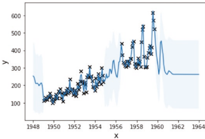
Figure 4-15. Visualizing the GP regression fit using composite kernels on both trend and seasonality
