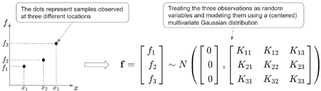
Figure 2-6. Modeling the three samples using a multivariate Gaussian distribution
