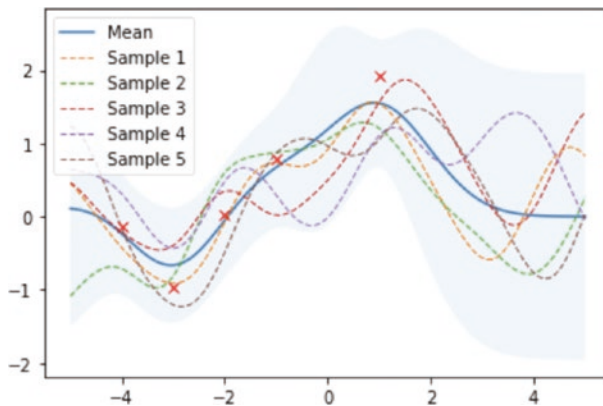
Figure 2-13. Drawing five samples from GP posterior based on noisy observations
