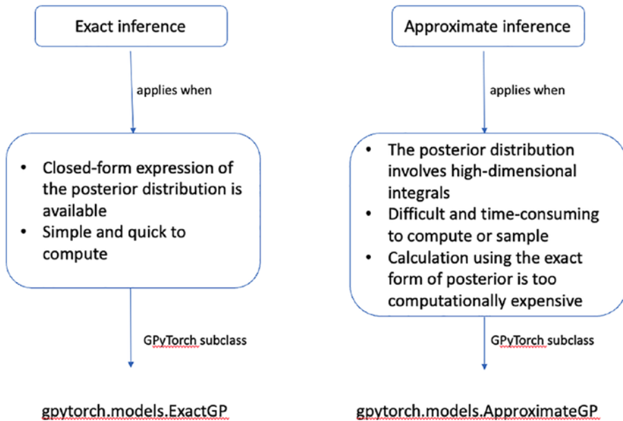
Figure 4-1. Comparing exact and approximate inference in GPyTorch
