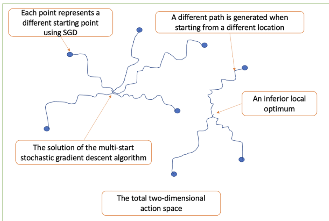
Figure 5-1. Illustrating the multi-start stochastic gradient descent algorithm in a two-dimensional action space, where multiple starting points are selected to generate different paths in parallel. The final solution is obtained by aggregating all endpoints upon convergence and taking the best candidate. Note that additional projection to the nearest sampling location is needed in the case of discrete action space
