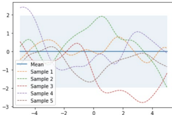
Figure 2-11. Five samples from the GP prior together with the mean function and 95% confidence intervals
