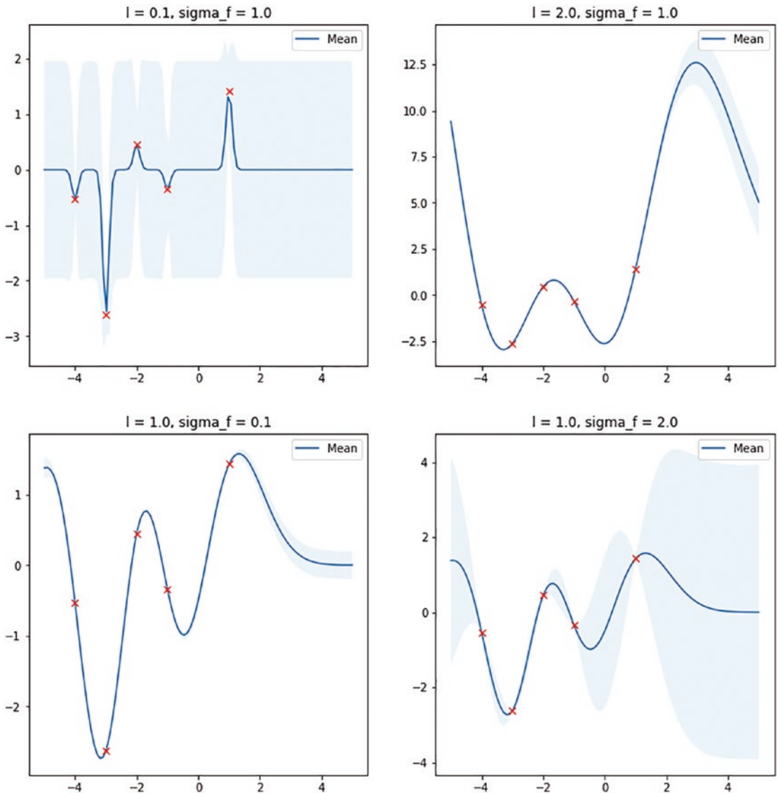
Figure 2-15. Illustrating four different settings of kernel parameters
