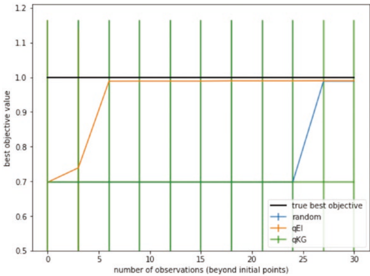
Figure 7-3. Comparing the performance of three search policies in identifying the optimal learning rate. The qEI acquisition function located the highest-performing learning rate in just two steps, while qKG exhibited more variation across all steps. The random strategy only caught up in the last few steps
