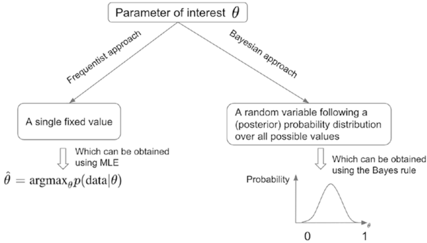
Figure 1-9. Comparing the frequentist approach and the Bayesian approach regarding the parameter of interest. The frequentist approach treats \theta as a fixed quantity that can be estimated via MLE, while the Bayesian approach employs a probability distribution which gets refreshed as more data is collected
