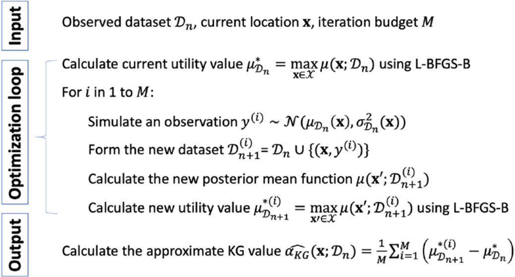
Figure 6-3. Illustrating the algorithm for calculating the KG value using Monte Carlo simulations
