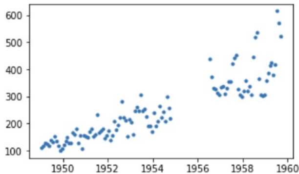
Figure 4-12. Visualizing the training set of the monthly airline passenger count data
