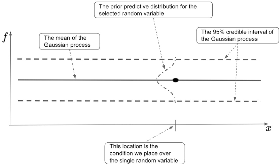
Figure 1-17. A sample prior belief of the Gaussian process represented by the mean and 95% credible interval for each location in the domain. Every objective value is modeled by a random variable that follows a normal prior predictive distribution. Collecting the distributions of all random variables could help us quantify the potential shape of the true underlying function and its probability
