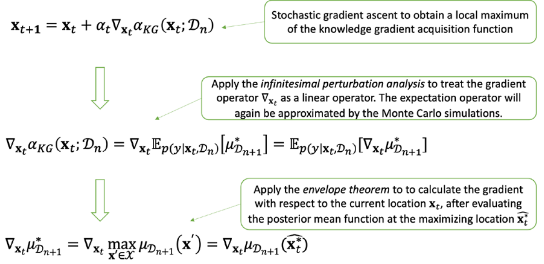
Figure 6-4. Illustrating the gradient calculation process for a given location
