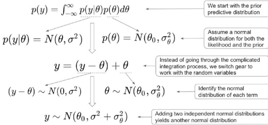
Figure 1-12. Derivation process of the prior predictive distribution for a new data point before collecting any observations, assuming a normal distribution for both the likelihood and the prior
