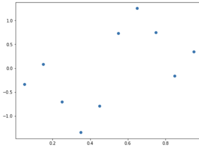
Figure 4-2. Visualizing the initial ten noisy observations
