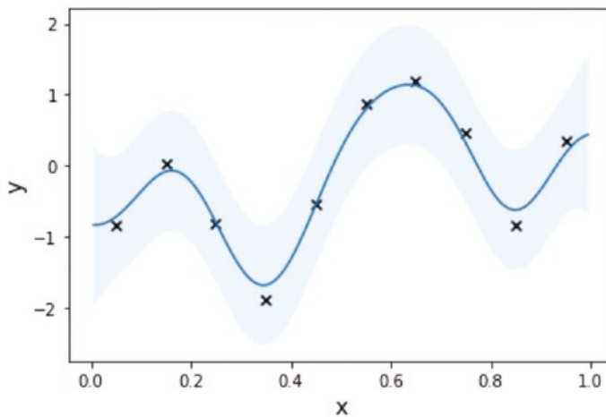
Figure 4-7. Visualizing the fitted GP model after overriding the noise variance
