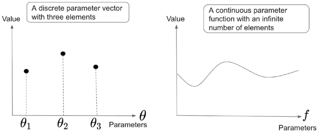
Figure 2-2. Comparing a discrete parameter vector (left) and a continuous parameter function (right), which is an extension from a limited set of parameters to an unlimited number of parameters embedded in a function
