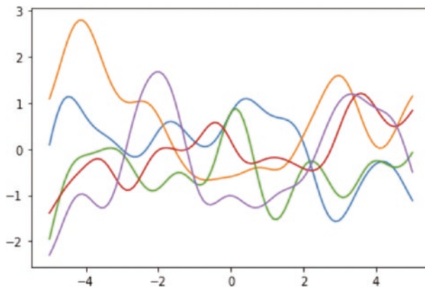
Figure 2-10. Drawing five random samples from a GP prior
