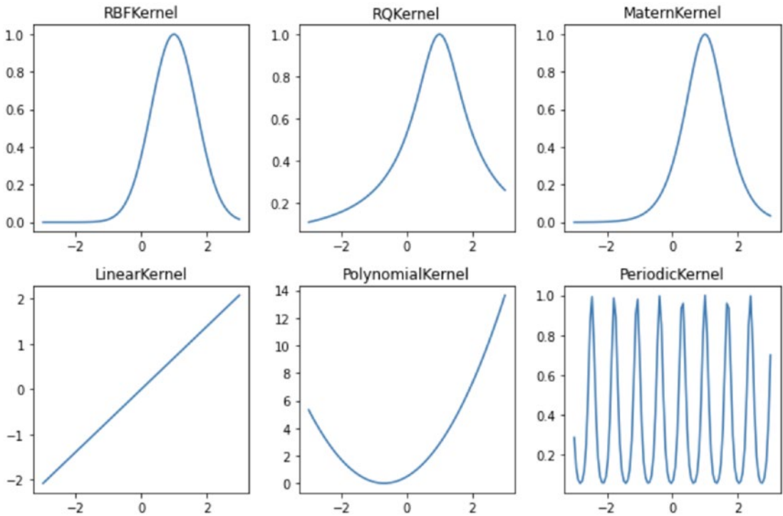
Figure 4-10. Visualizing different kernel functions
