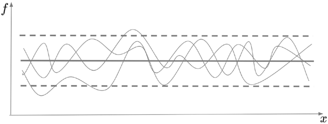
Figure 1-18. Three example functions sampled from the prior process, where majority of the functions fall within the 95% credible interval
