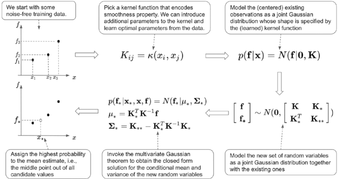
Figure 2-9. Obtaining the predictive distribution of new input locations using the Gaussian process. We start by defining and optionally optimizing a kernel function to encode what is observed from actual samples and what is believed using the prior. Then we model all variables as jointly Gaussian and obtain the conditional distribution for the new variables
