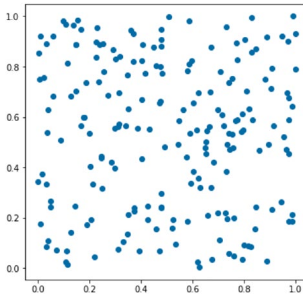
Figure 5-3. A space-filling design of 200 points generated following a uniform distribution, where the coverage is notably less sufficient than that covered by the Sobol sequences
