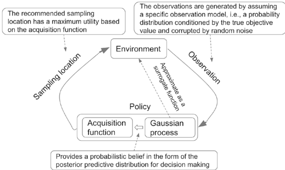
Figure 1-20. The full Bayesian optimization loop featuring an iterative interaction between the unknown (black-box) environment and the decision-making policy that consists of a Gaussian process for probabilistic evaluation and acquisition function for utility assessment of candidate locations in the environment
