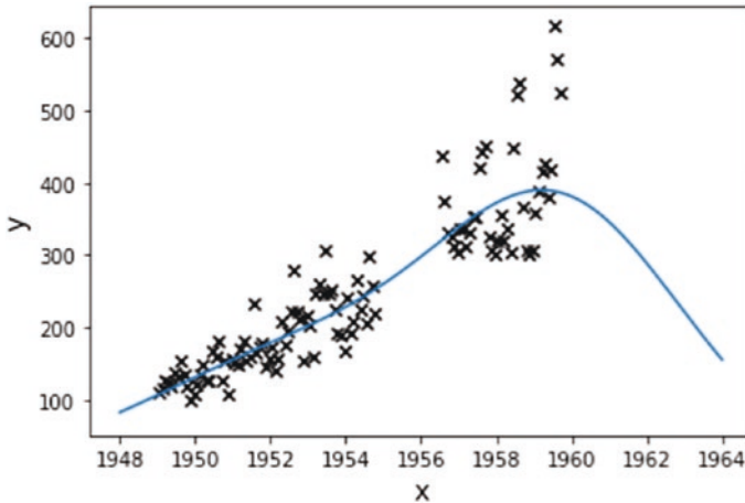
Figure 4-13. Visualizing the GP regression fit using the RBF kernel
