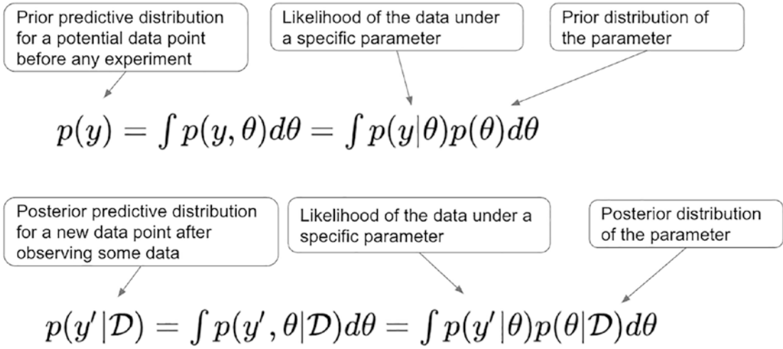
Figure 1-11. Definition of the prior and posterior predictive distributions. Both are calculated based on the same pattern of a weighted sum between the prior and the likelihood
