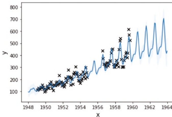
Figure 4-16. Visualizing the GP regression fit using composite kernels on the trend, seasonality, and heteroscedastic noise
