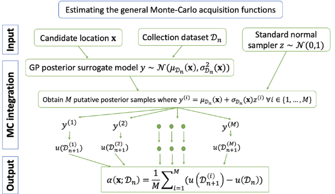
Figure 6-2. Schematic of optimizing general Monte Carlo acquisition functions
