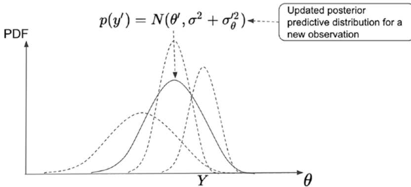
Figure 1-16. Illustrating the posterior predictive distribution if we acquire another observation from the system/environment under study. The posterior predictive distribution shares the same mean as the posterior distribution of \theta but now has a larger spread due to uncertainty from both \theta and the observation model
