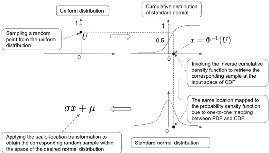
Figure 2-5. Obtaining a random sample from the desired univariate Gaussian distribution based on three steps: sampling from a uniform distribution, converting to the corresponding input of the CDF (or PDF) using the inverse cumulative function, and applying the scale-location transformation to convert the random sample to the space of the normal distribution with the desired mean and variance
