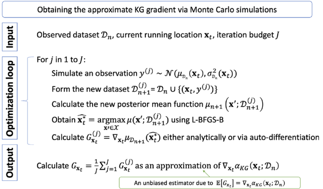
Figure 6-5. Illustrating the algorithm for calculating the gradient of KG using Monte Carlo simulations
