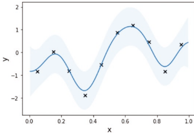
Figure 4-9. Fitting GP regression model with fixed noise variance and optimized length scale
