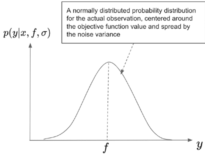
Figure 1-6. Assuming a normal probability distribution for the actual observation as a random variable. The Gaussian distribution is centered around the objective function f value evaluated at a given location x and spread by the variance of the noise term
