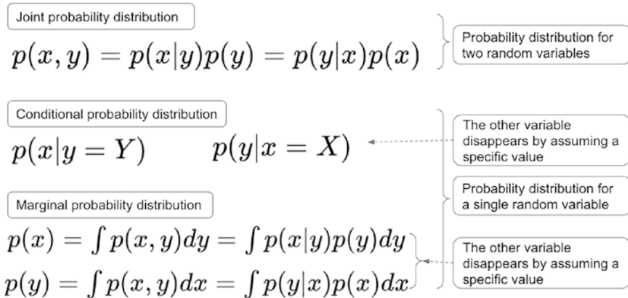
Figure 1-10. Three common probability distributions. The joint probability distribution represents the probability distribution for two or more random variables, while the conditional and marginal probability distributions generally refer to the probability distribution for one random variable. The conditional distribution represents the probabilities of a random variable by assuming/conditioning a specific value for other variables, while the marginal distribution converts a joint probability to a single random variable by integrating out other variables
