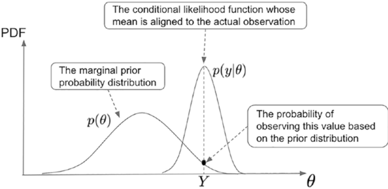
Figure 1-14. Illustrating the prior distribution and the likelihood function, both following a normal distribution. The mean of the likelihood function is equal to the actual observation due to the effect of conditioning
