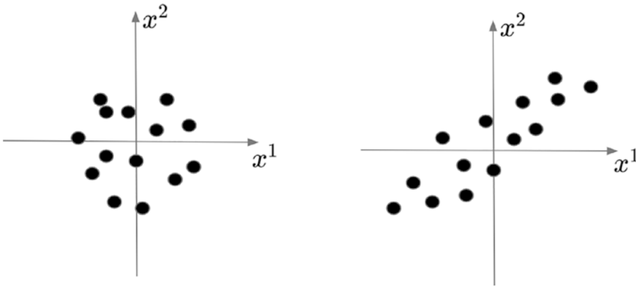
Figure 2-3. Illustrating two possible distributions of points on a plane centered at the origin. These points could be equally distributed around the origin (left) or distributed with a systematic bias (right)
