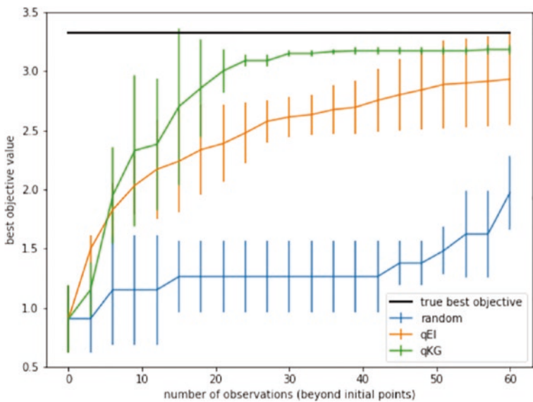
Figure 7-1. Comparing the performance of three search policies: qEI , qKG , and random search. The qKG acquisition function has the best performance due to its less myopic nature, while qEI only dominates in the first step and starts to perform inferior to qKG due to its myopic nature. Both qEI and qKG perform better than the random policy, showing the benefits of employing this side computation in the global optimization exercise
