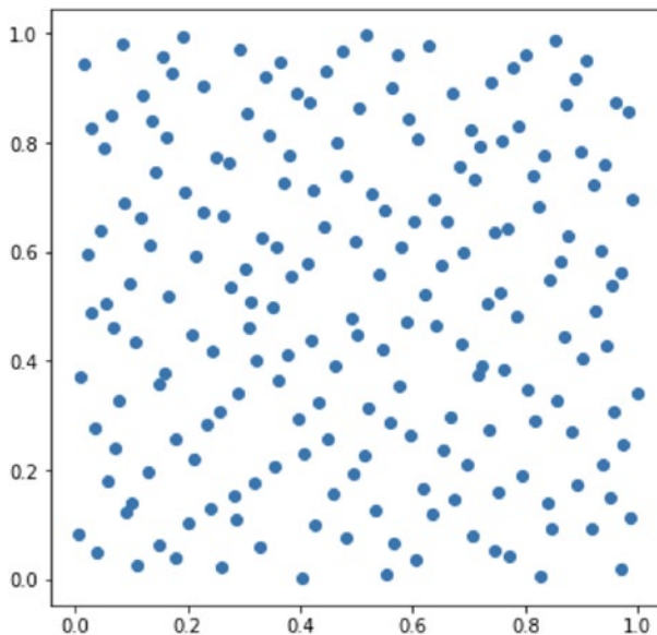
Figure 5-2. Sobol sequences that consist of 200 quasi-random points in a two-dimensional space. The points appear to be evenly distributed across the whole space, providing better estimates and faster convergence in optimization tasks
