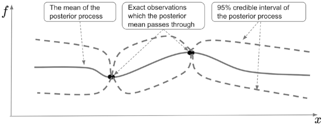
Figure 1-19. Updated posterior process after incorporating two exact observations in the Gaussian process. The posterior mean interpolates through the observations, and the associated variance reduces as we move nearer the observations
