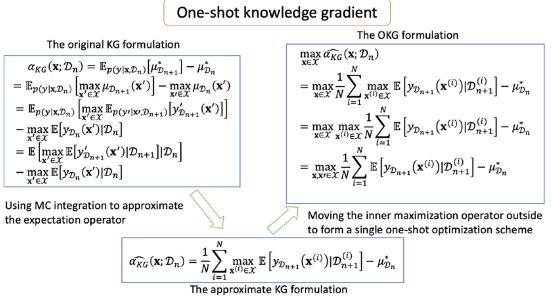
Figure 6-9. Illustrating the one-shot knowledge gradient formulation
