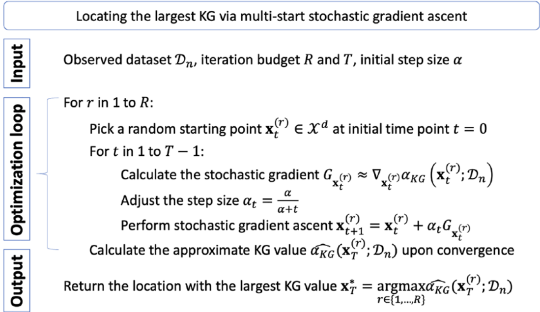
Figure 6-7. Illustrating the algorithm for locating the largest KG for sequential sampling using multi-start stochastic gradient ascent
