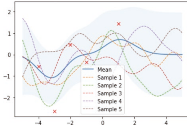
Figure 2-14. A wider confidence interval across the whole input domain given a lower signal-to-noise ratio
