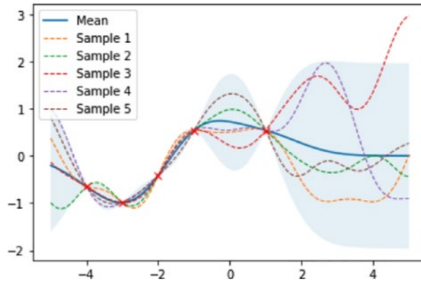
Figure 2-12. Drawing five samples from GP posterior based on noise-free observations
