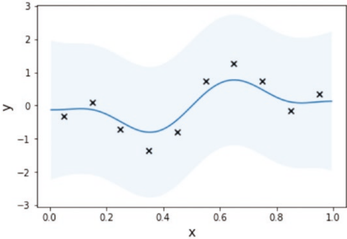
Figure 4-5. GP regression model after setting the length-scale parameter manually
