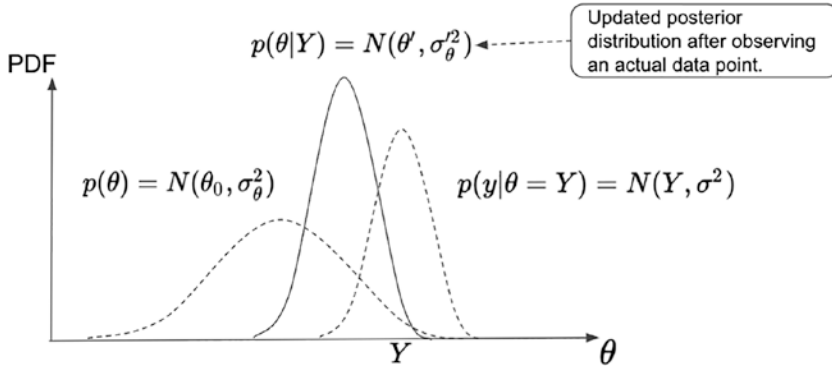
Figure 1-15. Deriving the posterior distribution for \theta using Bayes' rule. The updated mean \theta' is now between the prior mean \theta_0 and actual observation Y , suggesting an alignment between subjective preference and reality
