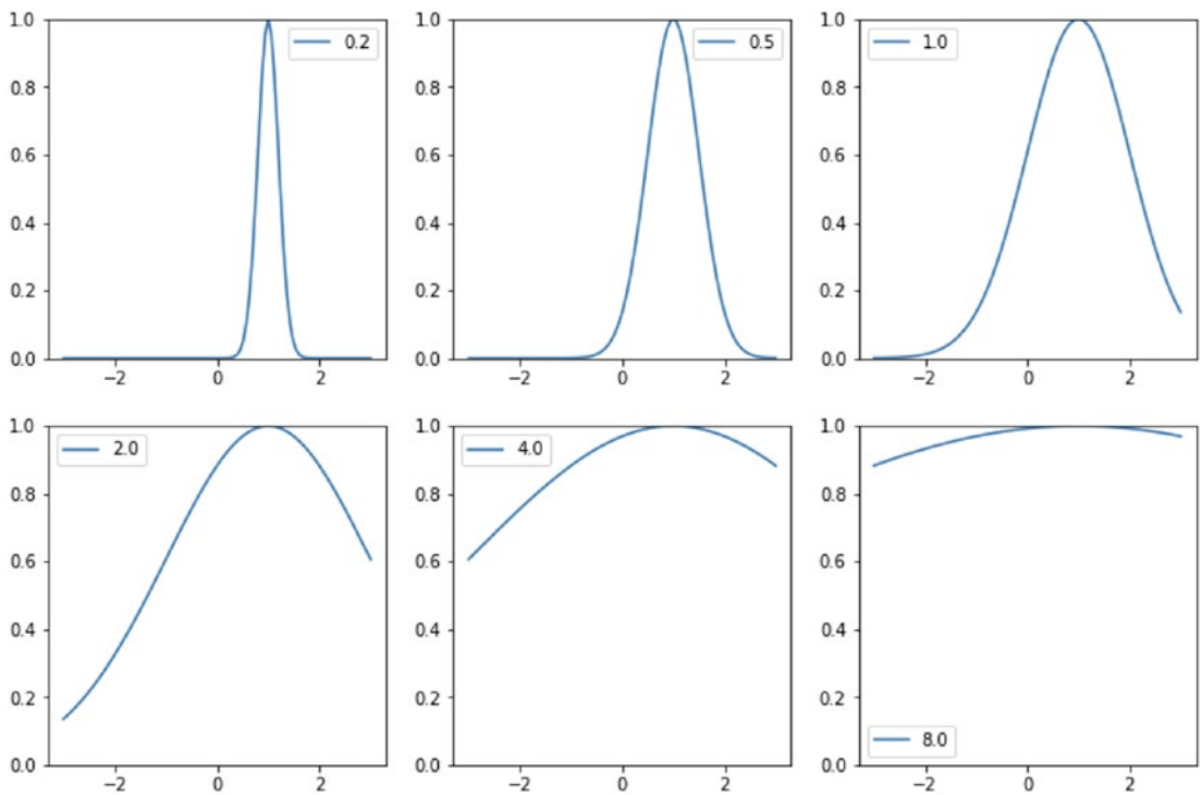
Figure 4-4. Visualizing the kernel function under different length-scale parameter settings
