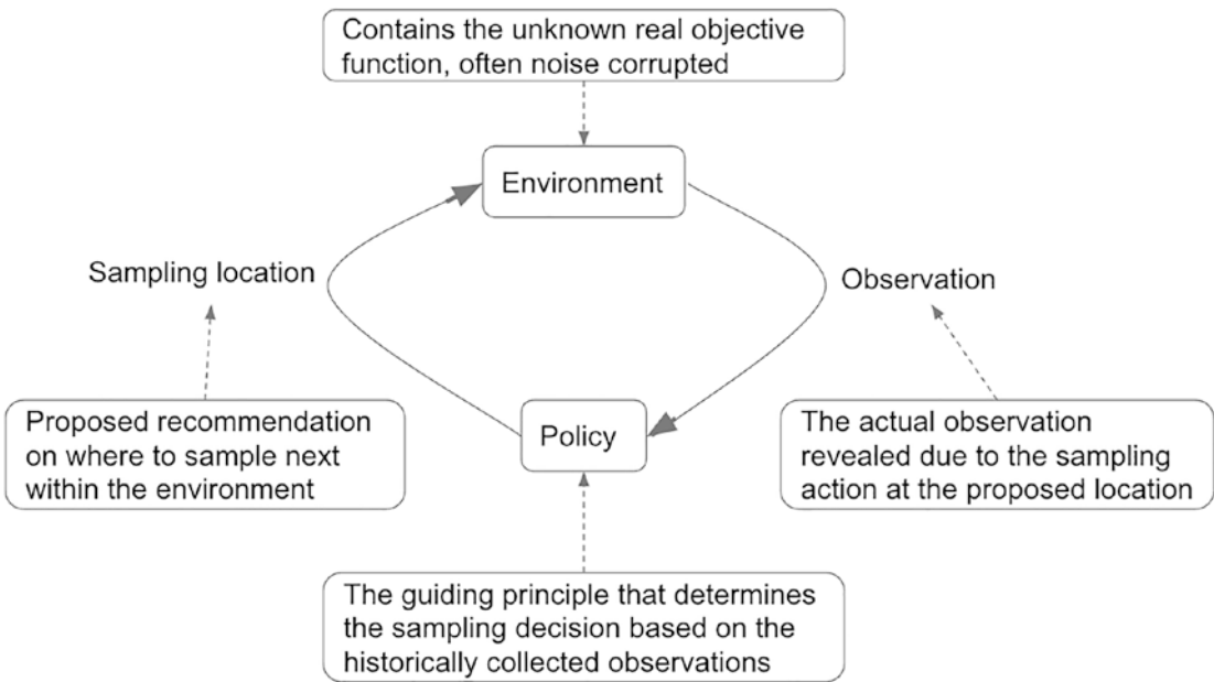
Figure 1-1. The overall Bayesian optimization process. The policy digests the historical observations and proposes the new sampling location. The environment governs how the (possibly noise-corrupted) observation at the newly proposed location is revealed to the policy. Our goal is to learn an efficient and effective policy that could navigate toward the global optimum as quickly as possible
