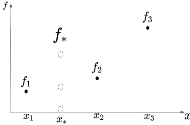
Figure 2-8. Three possible values of f_* (dash circles) for a new input location x_* . Based on the smoothness assumption encoded in the kernel/covariance function, we would intuit the middle point to be the most likely candidate
