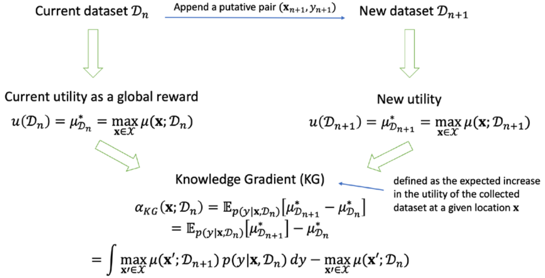
Figure 6-1. Illustrating the knowledge gradient acquisition function
