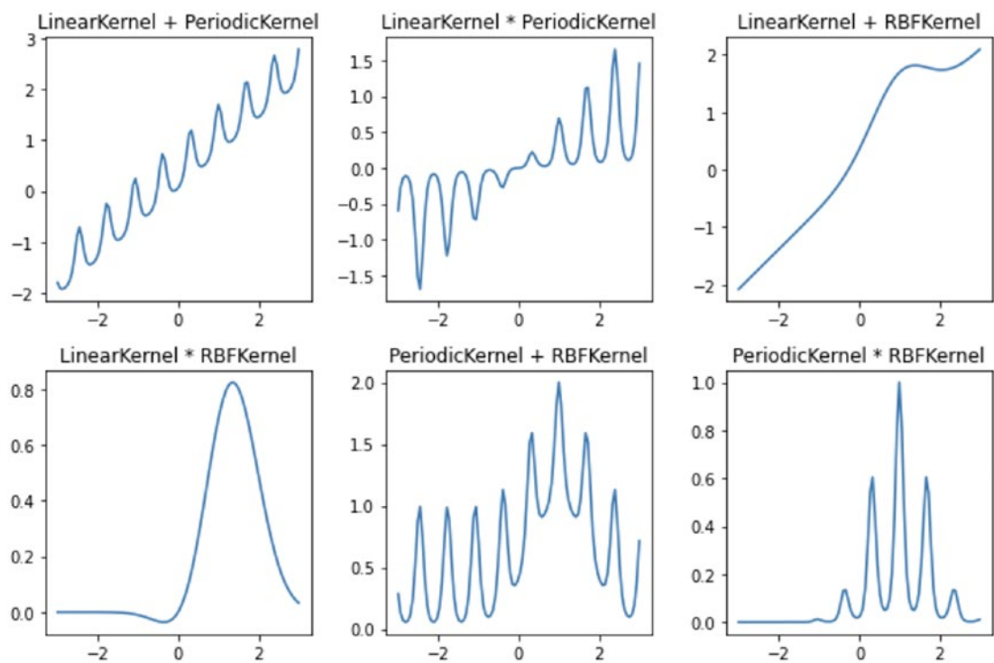
Figure 4-11. Visualizing different combined kernels
