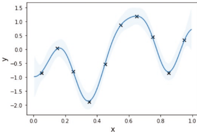
Figure 4-8. Visualizing the GP model fitted with increased noise variance
