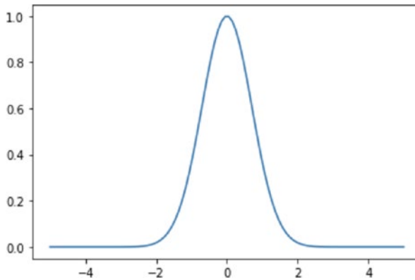
Figure 2-7. Visualizing the squared exponential kernel function
