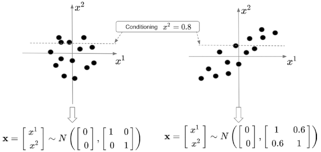
Figure 2-4. Illustrating the bivariate Gaussian distribution for the two scenarios. The covariance entries on the left are set to zero to represent the fact that the variables are uncorrelated, while the covariance entries are 0.6 due to a positive correlation on the right
